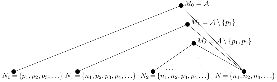
Figure 7: A family of curb models which is not well-founded ( \mathcal{A} = \{p_i, n_i \mid i = 1, 2, \dots\} )
