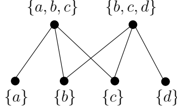
Figure 6: The Weak LUB property does not imply the LUB property
