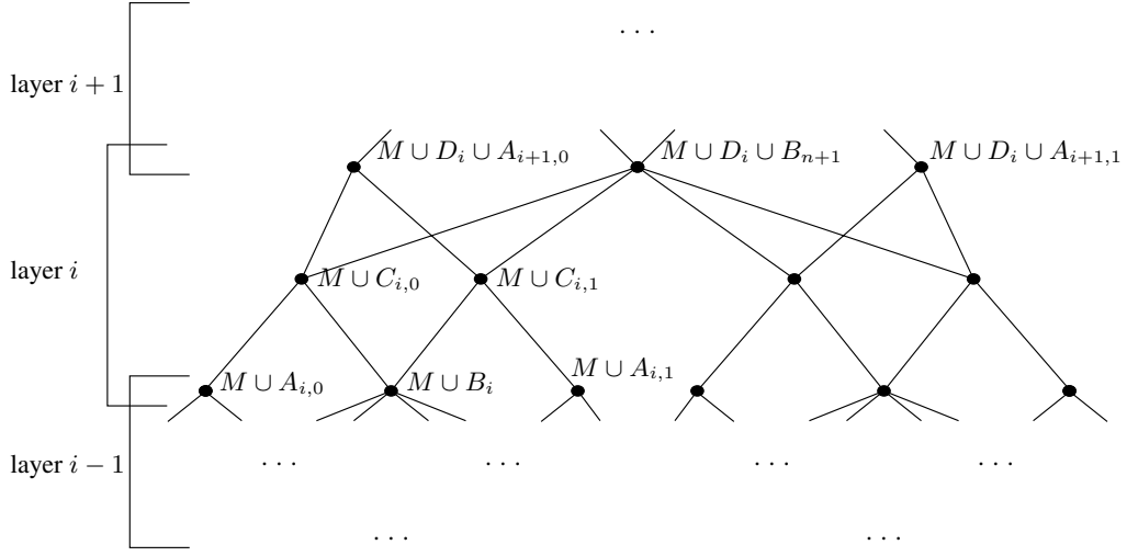
Figure 10: Layers in \text{mod}(\varphi_n)
