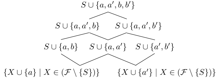
Figure 8: Cloning a family \mathcal{F} with unique maximal model S
