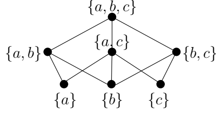
Figure 4: Set of curb models whose ranks are not strictly decreasing along chains
