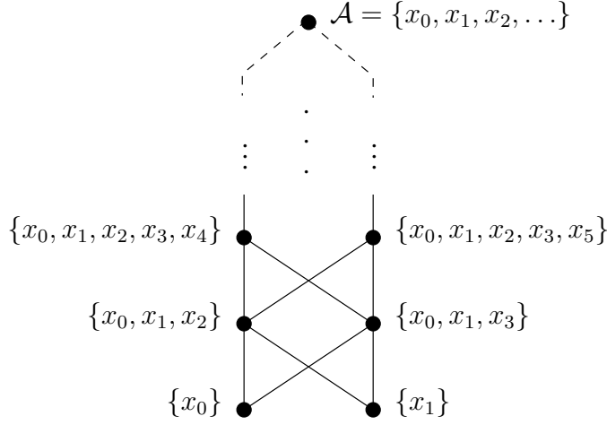
Figure 5: The infinite tower
