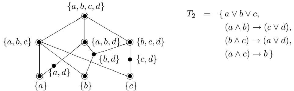
Figure 3: The party example
