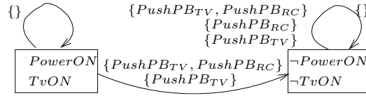
Figure 2: Transition diagram of D^{(2)} = D_u \cup Q \cup \{(2)\} .
