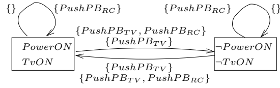
Figure 1: A transition diagram.
