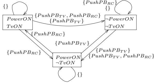
Figure 3: Transition diagram of D^{(3)} = D_u \cup Q \cup \{(1)\} .
