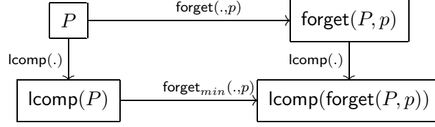
Figure 1: Commuting logic program completion and forgetting
